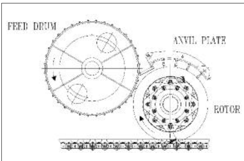
Figure 3. The in-line shredder
