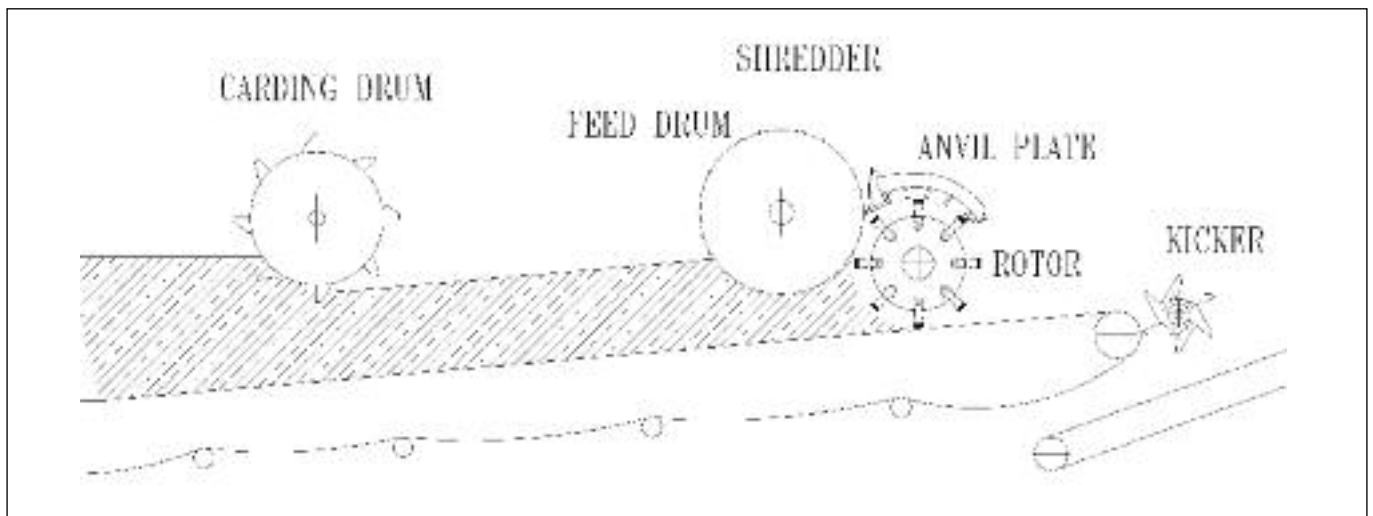
Figure 4. A typical in-line shredder installation
