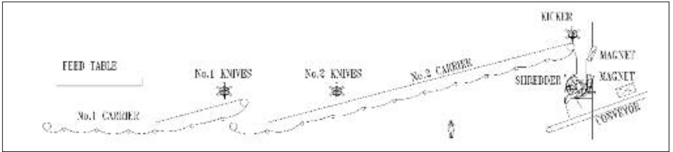
Figure 2. An alternative cane preparation station with contra-rotating knives
