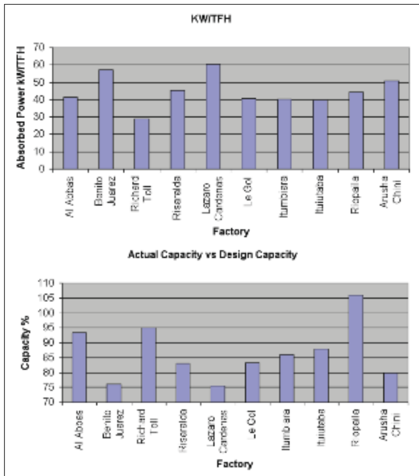
Figure 7. Power consumption and capacity of installed in-line shredders
